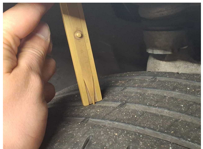
Damage 3: Wheel / tyres: Tyre - front right side - Worn - Replace
