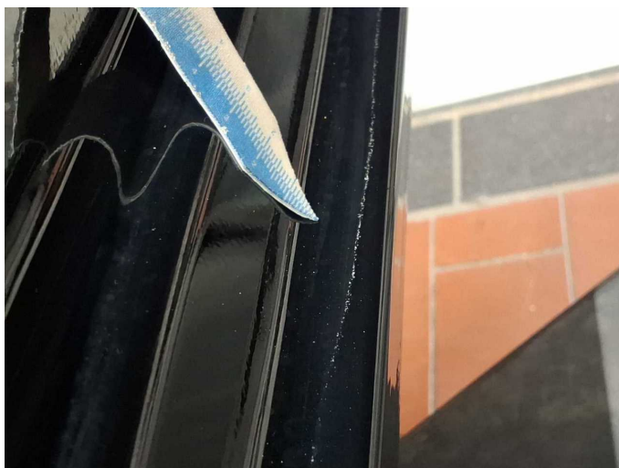
Damage 5: Sill - right side: Sill (Lackläufer) - Unprofessionally repaired - Repair and paint
