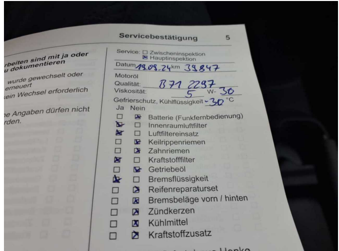
Figure 14: Documents
