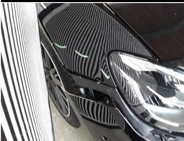
Damage #8: Mudguard - right side: Mudguard - right side - Deformed - Repair and paint
