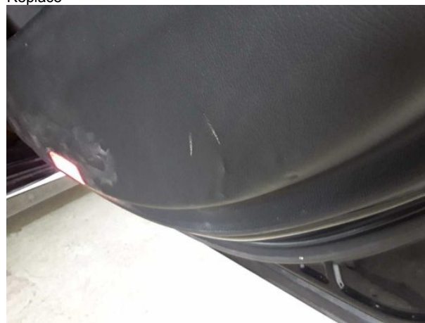
Damage #6: Trim / covers: Door trim - rear right side - Deformed - Replace
