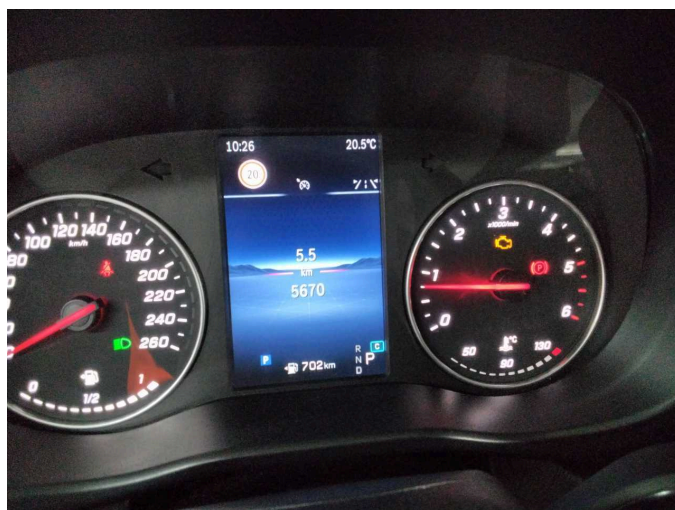
Damage 2: Instrument panel: Indicator light (Motorkontrolle) - on - Perform diagnosis
