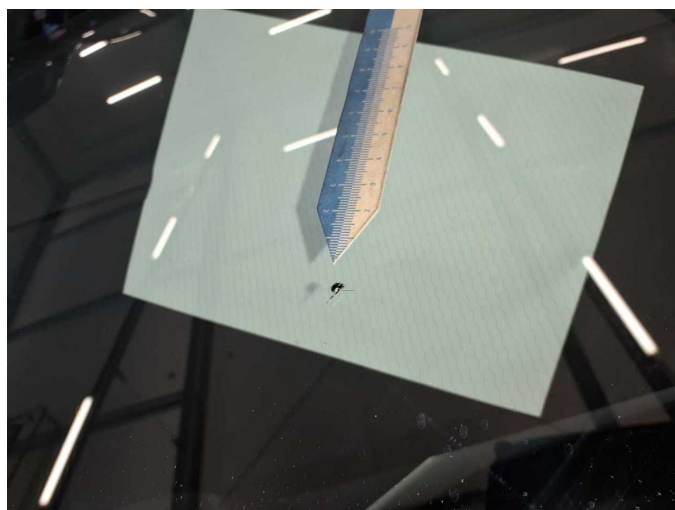
Damage 5: Vehicle glazing: Windscreen (Beheizbare Frontscheibe) - Stone chips - Replace
