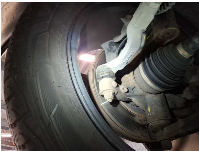
Damage 14: Steering system: Tie rod end (Links--> Achsvermessung) - Broken / torn - Replace
