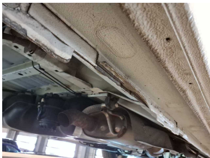
Damage 12: Sill - right side: Sill - Deformed - Smart repair
