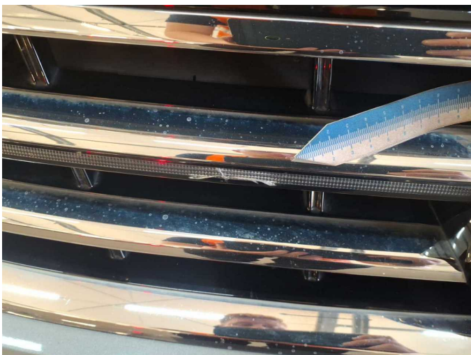
Damage 6: Bonnet: Air grille - Broken / torn - Replace
