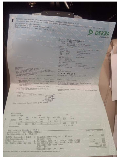
Figure 16: Documents
