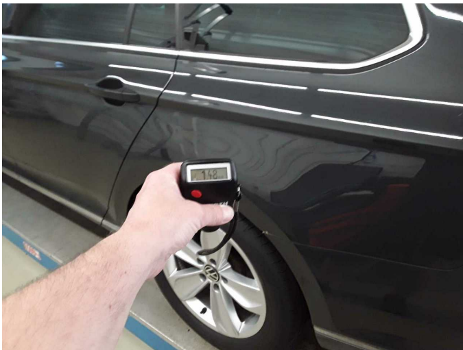
Side panel - rear left side: 1,480 \mu\text{m}
