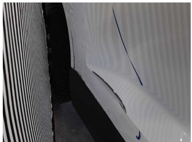
Damage #24: Door - rear right side: Door - Deformed - Replace
