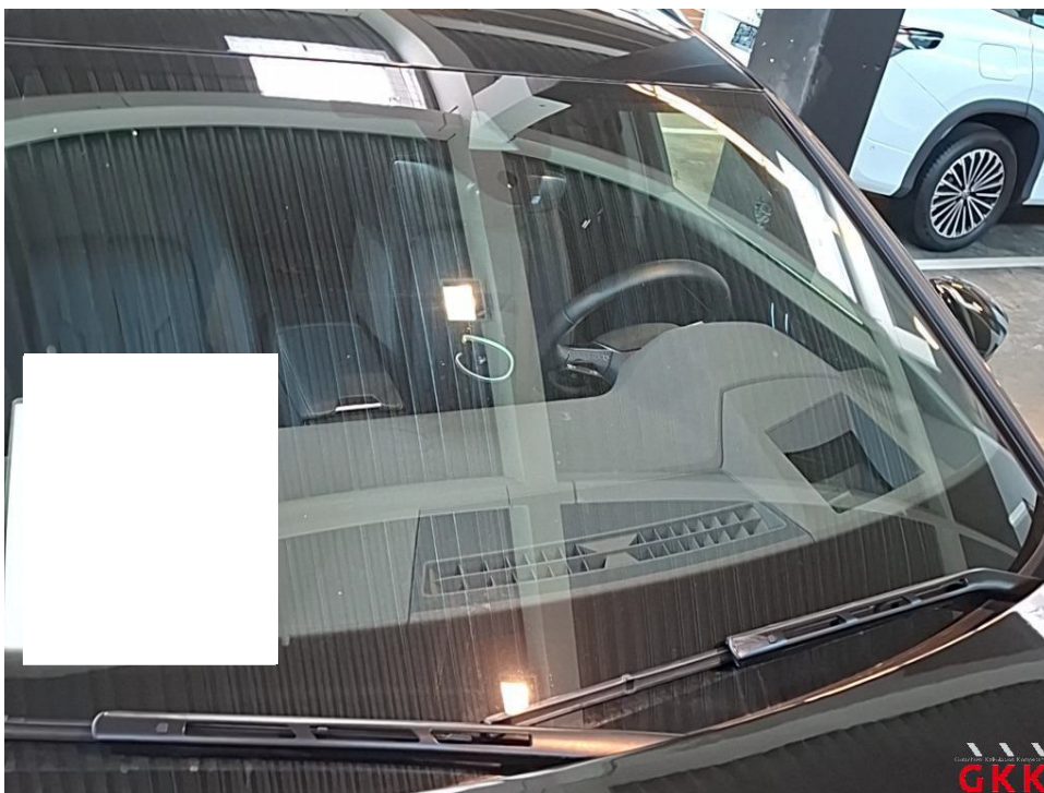
Picture 18 front screen, with rain sensor and frontcamera, chipping, repair
