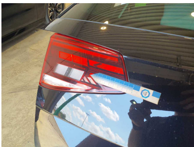
Damage 9: Tail light: Tail lamp - left side - Broken / torn - Replace
