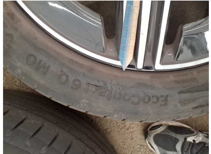
Damage 1: 2nd wheel set: 1 tyre - Broken / torn - Replace
