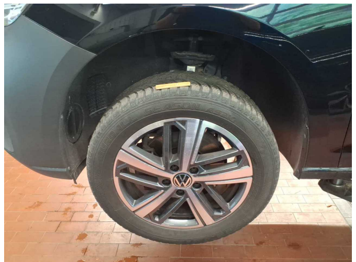
Damage 6: Wheel / tyres: Tyre - front (Unter 4mm) - Does not meet the leasing specifications - Replace
