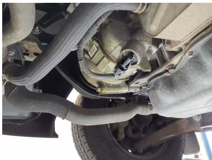
Damage 3: Air-conditioning system: Air-conditioning system (Kompressor, Mehrkosten möglich) - Leaking - Perform diagnosis
