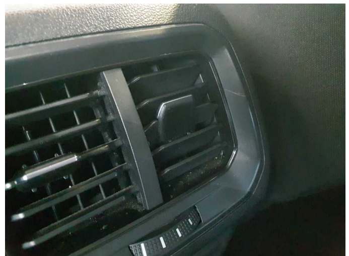
Damage 6: Instrument panel: Air nozzle - centre - Damaged - Replace
