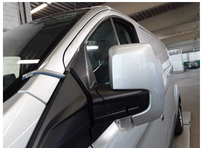
Damage 3: Wing mirror - left side: Mirror housing - Damaged - Replace
