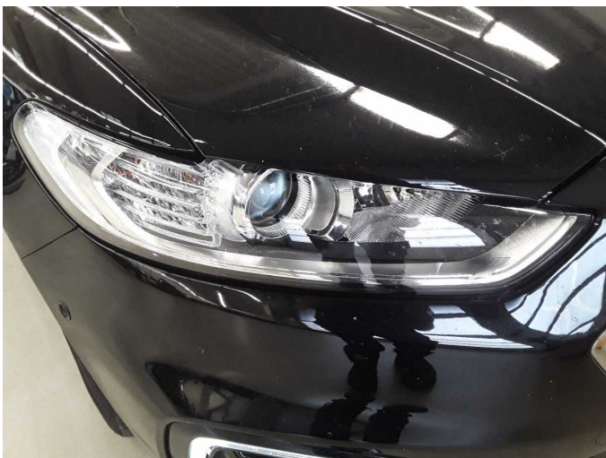
Damage 3: Headlight: Headlight - right side (Leuchtmittel H7) - Non-operational - Perform diagnosis
