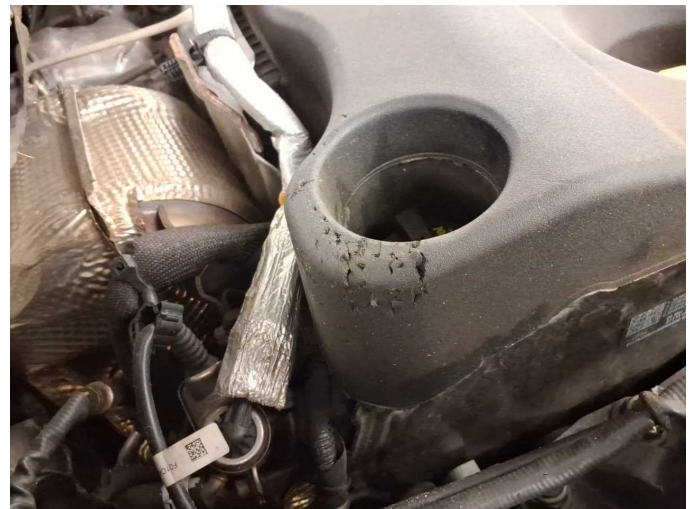
Damage 8: Engine: Engine cover - Damage caused by marten / rodent - Replace
