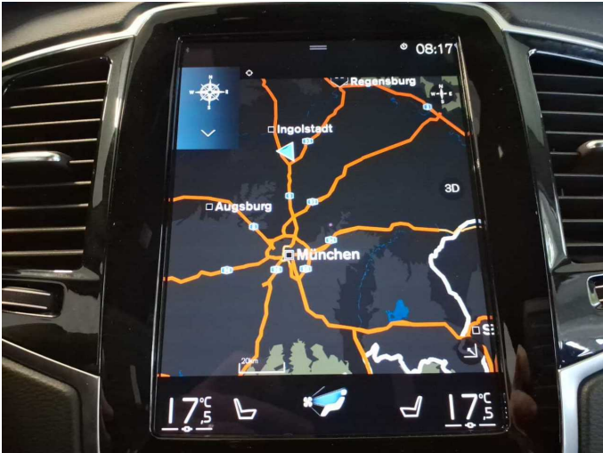
Figure 18: Navigation
