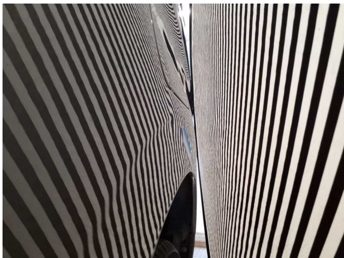
Damage 11: Side panel - rear left side: Side panel (wellig-teilweise) - Unprofessionally repaired - Repair and paint
