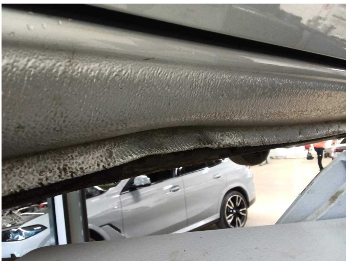
Damage 3: Sill - left side: Sill - Deformed - Repair and paint
