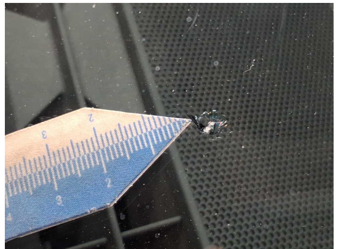
Damage 11: Vehicle glazing: Windscreen - Stone chips - Replace
