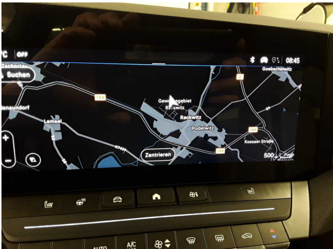
Figure 24: Navigation
