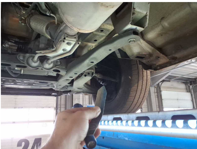
Damage 2: Drive train: Sleeve prop shaft - front right side - Broken / torn - Replace
