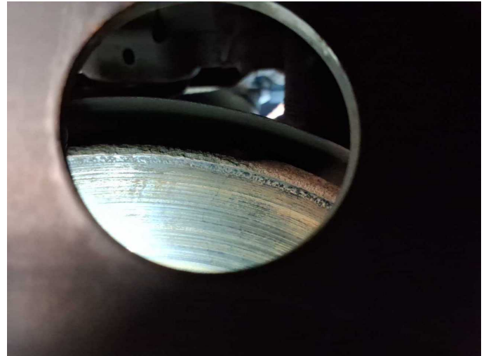
Damage 10: Braking system: Brake discs and pads - rear (Tragbild mangelhaft, Rost) - Worn - Replace
