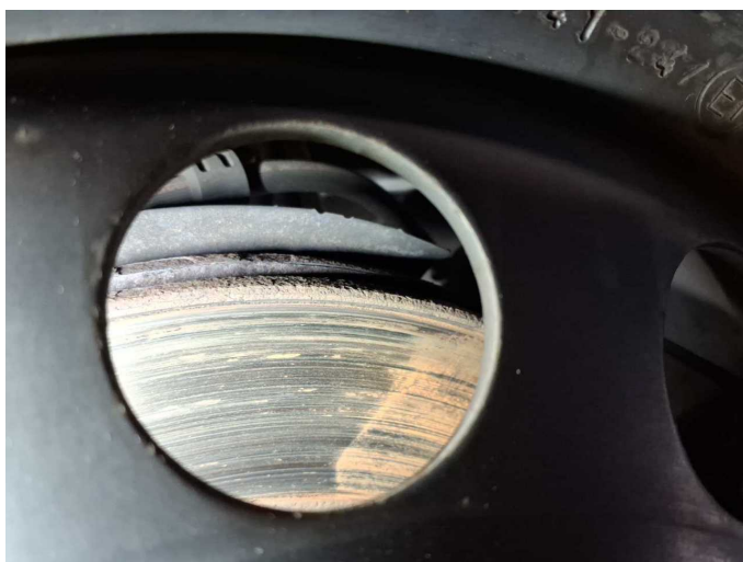
Damage 9: Braking system: Brake discs and brake pads - front (Tragbild mangelhaft, Rost) - Worn - Replace
