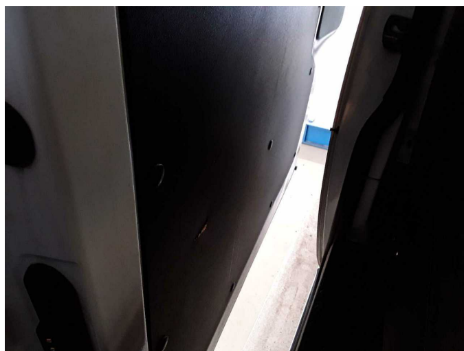
Damage 8: Sliding door, right: Trim washable - lower - Broken / torn - Replace
