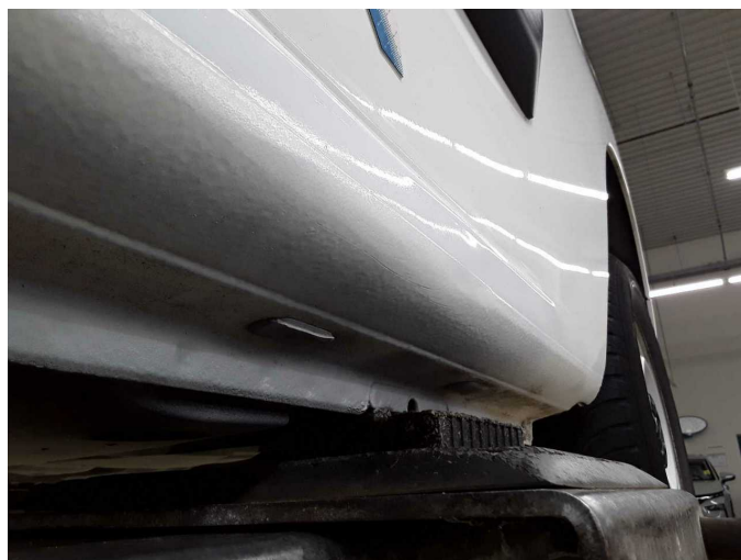
Damage 13: Sill - left side: Sill - Unprofessionally repaired - Repair and paint
