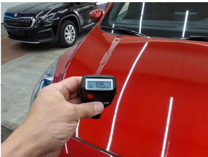
Repainting 1: Boot lid / rear door, Bonnet, Side panel - rear left side, Door - rear left side
