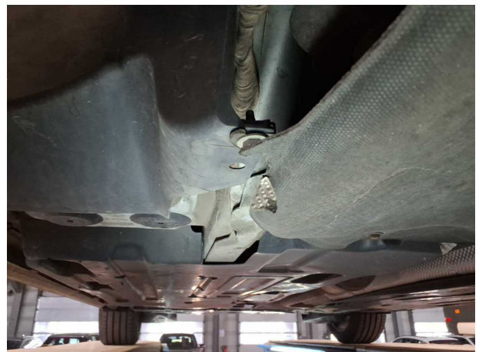
Damage 12: Engine: Engine cowling - lower - Broken / torn - Replace
