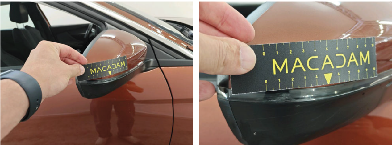
Mirror side repeater R Scratch(es) Replace Right
