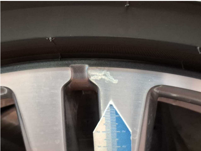
Damage 4: Wheel / tyres: Alloy rim - front left side - Corrosion - Replace
