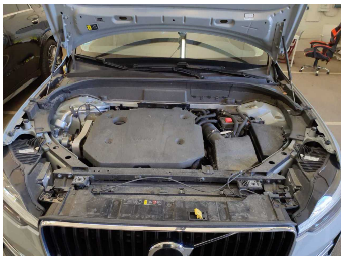
Damage 1: Engine: Engine cover (Dichtung L + R) - Damage caused by marten / rodent - Replace
