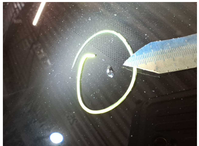
Damage 9: Vehicle glazing: Windscreen with lane departure assistant (durch Steinschlag) - Broken / torn - Replace
