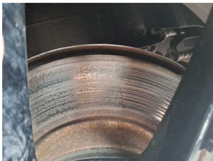
Damage 8: Braking system: Brake discs and pads - rear (Tragbild mangelhaft. Riefen.) - Corrosion - Replace
